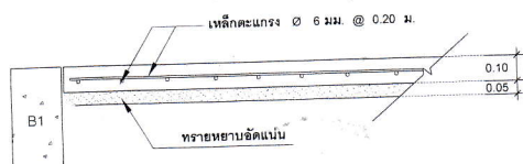
DETAIL S1
