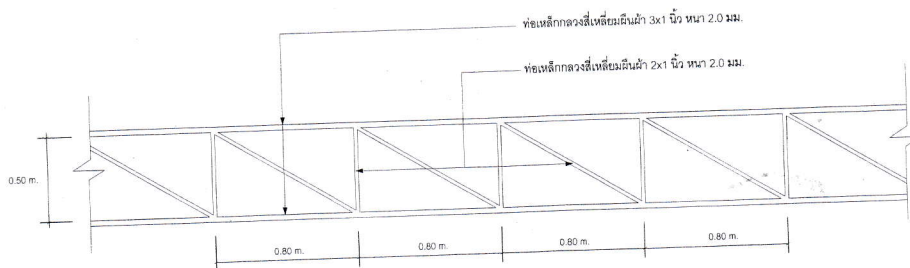
DETAIL Truss
