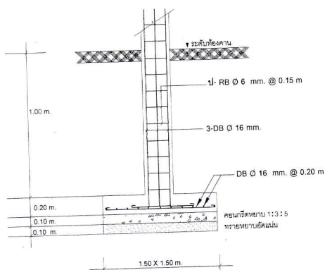
DETAIL F
