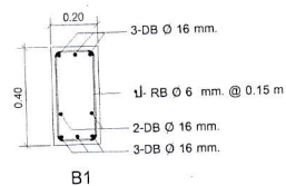
DETAIL BEAM
