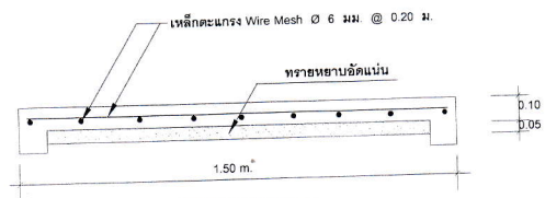
DETAIL S2
